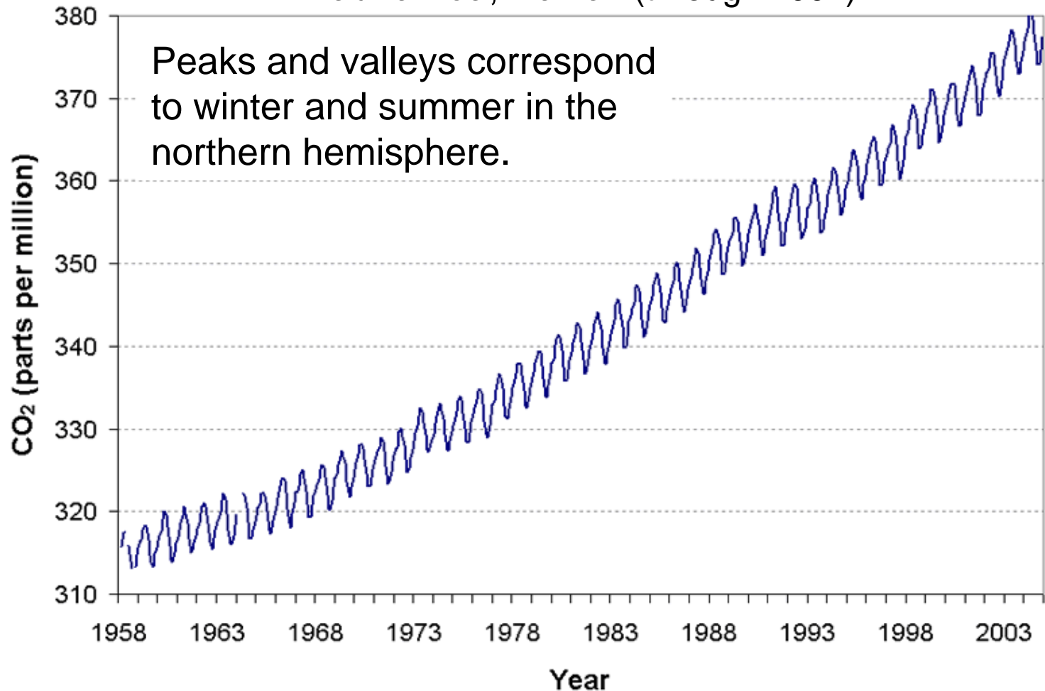
Mauna Loa, Hawaii (through 2004)
